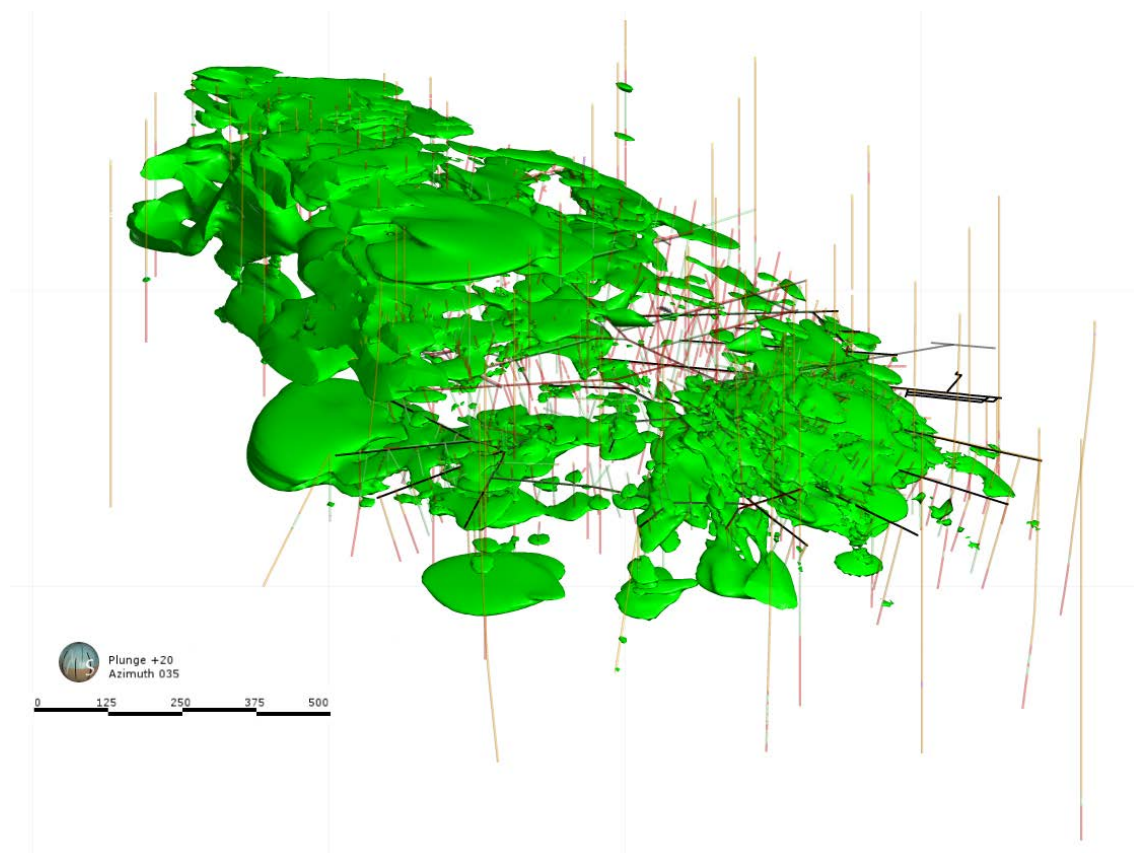
Figure 1 Spatial distribution of greisen bodies in the Cinovec deposit, looking in a North East direction. The greisen (shaded green) is overlain by barren rhyolite (not shown) and hosted by variably altered granite (not shown). Note traces of drill holes and UG workings.
